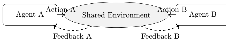
Figure 1: Generic model of unaware adversaries: agents act on a shared environment, receive feedback only via its state, and have no direct communication or awareness of their mutual antagonism.
